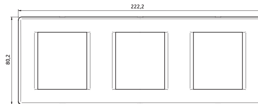
Multi-gang frame 3x2M horizontal
