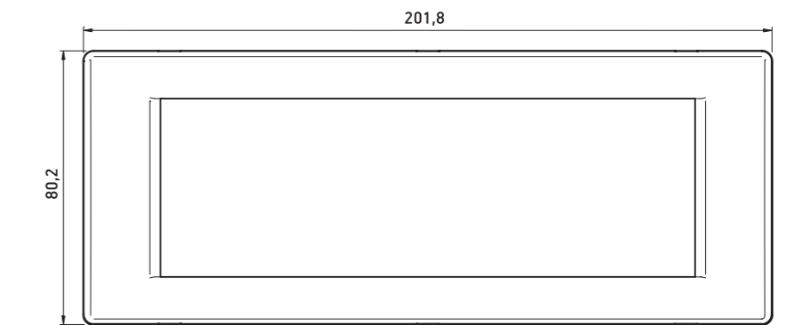
Maska sedmostruka Seven-gang frame
